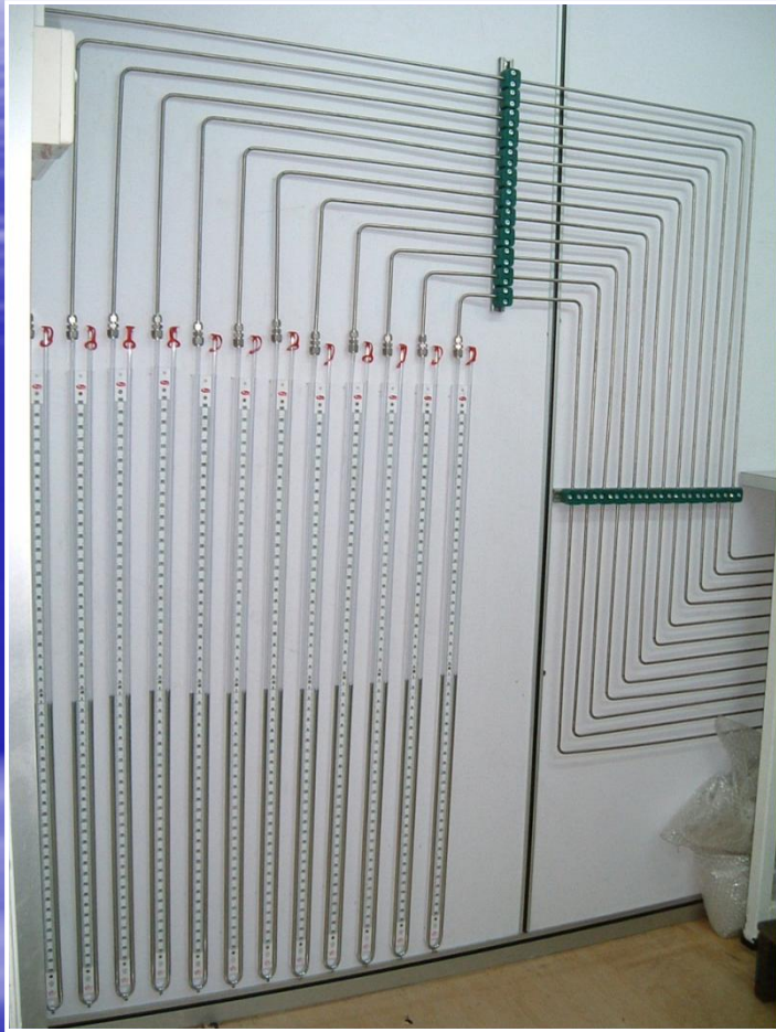
MERCURY U-TUBES
